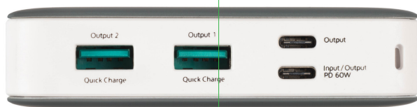
USB-C PD IN/OUTPUT
